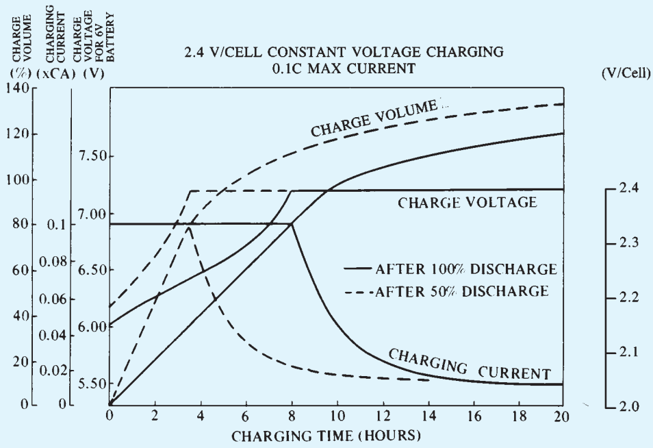
Figure 9. CHARGING CHARACTERISTICS
